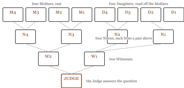
FIG. 2. THE SHIELD. Sixteen random marks become four Mothers; the Mothers are transposed into four Daughters; and the eight are folded downward in pairs to two Witnesses and one Judge. Every step below the Mothers is determined; there is no judgement in the arithmetic, only in the question and the reading. Drawn for this book.
