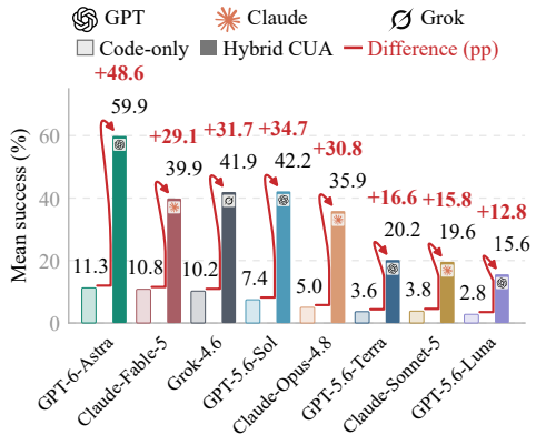
Figure 1: CUA-SWE benchmark overview and Frontier agents performance. Left: Agents inspect screenshots, interact with applications, and edit code; independent tests check their repairs. Right: Mean task success of Code-only and Hybrid CUA agents across four equally weighted domains. Red labels show the Hybrid CUA gain in percentage points.
