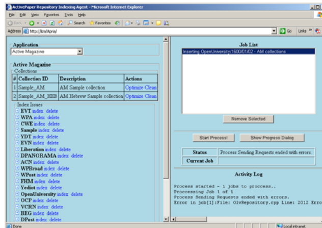
Figure 64: Apria Window in Internet Explorer
