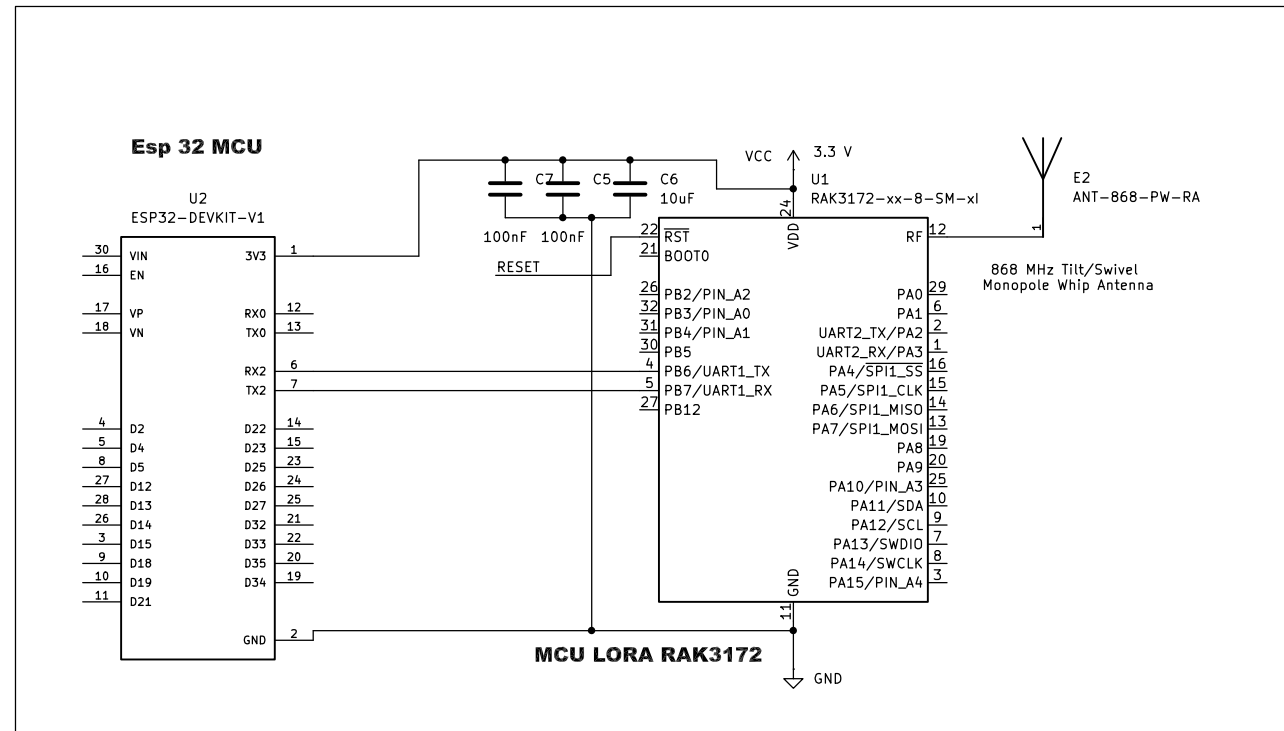
LoRa Reciver Side (MQTT Bridge side ) Circuit
