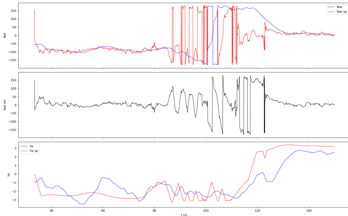
Annex B, t = 33 –150 s: first leg flown in reverse ( v_x setpoint \approx -2.3 m/s), then the turnaround — the yaw setpoint (red) thrashes across \pm 180^\circ while the vehicle grinds through a 261^\circ rotation in 45 s.
