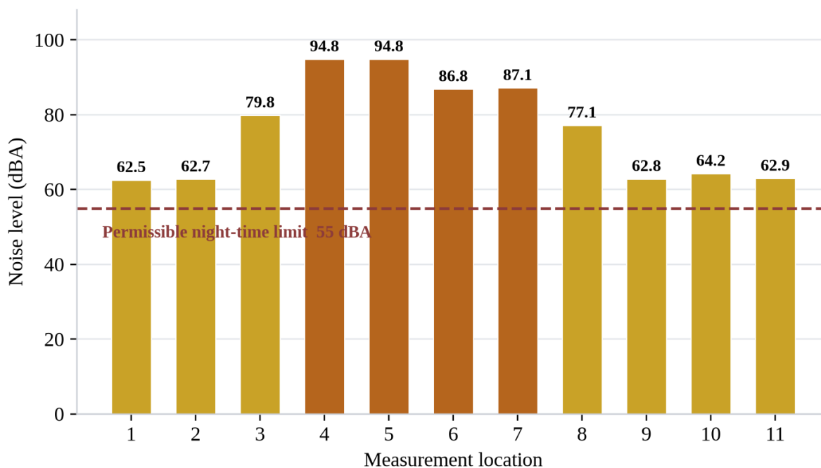
Figure 21. Recorded noise levels against the permissible night-time limit, Peuto Dela Torres Compound, 14 September 2026
