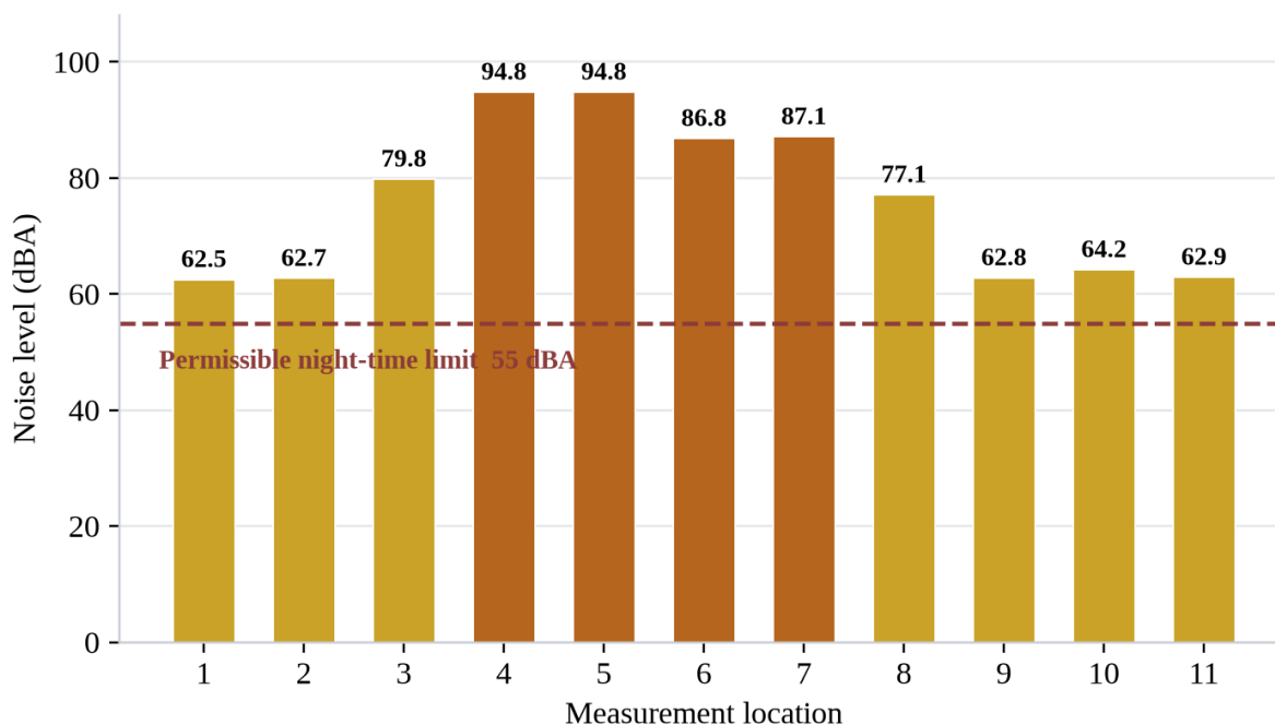
Figure 18. Recorded noise levels against the permissible night-time limit, Peuto Dela Torres Compound, 14 September 2026
