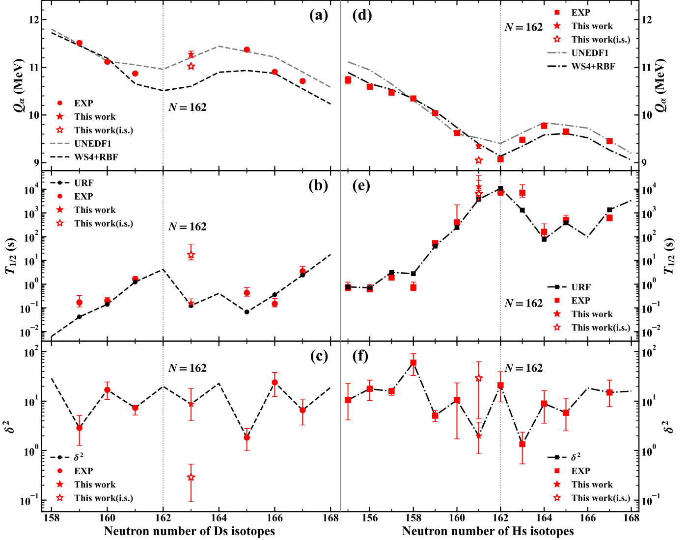
Figure 4: Systematics of Q_\alpha , T_{1/2} , and reduced \alpha -decay width \delta^2 for the Ds and Hs isotopic chains. Panels (a)–(c) correspond to Ds isotopes and panels (d)–(f) correspond to Hs isotopes. The upper, middle, and lower rows show Q_\alpha , T_{1/2} , and \delta^2 , respectively, as functions of neutron number. Experimental values are compared with the UNEDF1 and WS4+RBF calculations in the Q_\alpha panels and with the URF values in the half-life panels. The filled stars denote the branches assigned in the present work, and the open stars denote the tentative isomeric branches. The vertical dotted lines indicate N = 162 .
