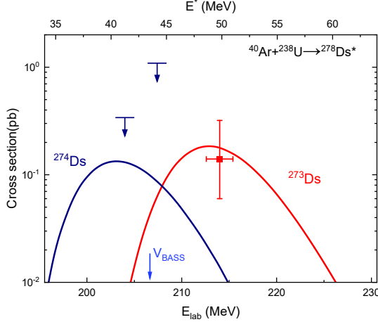
Figure 5: Measured cross section and upper limits for the ^{40}\text{Ar} + ^{238}\text{U} \rightarrow ^{278}\text{Ds}^* reaction. The curves show the calculated excitation functions for the 4n and 5n channels leading to ^{274}\text{Ds} and ^{273}\text{Ds} , respectively. The lower horizontal axis gives the laboratory beam energy, and the upper axis gives the corresponding average excitation energy of the compound nucleus. The arrow marked V_{\text{BASS}} indicates the Coulomb barrier estimated with the BASS prescription.
