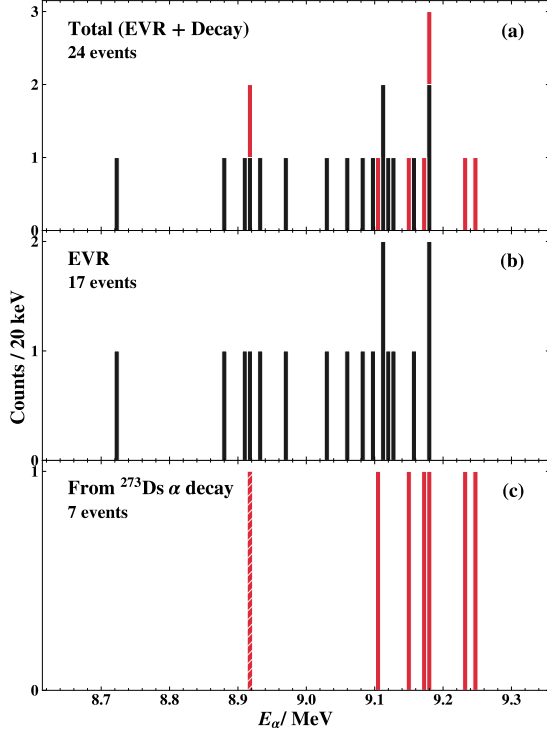
Figure 3: Measured \alpha -particle energy distribution for events assigned to ^{269}\text{Hs} . Panel (a) shows the full event sample, panel (b) shows the directly produced evaporation-residue sample, and panel (c) shows the events populated through the \alpha decay of ^{273}\text{Ds} . The hatched bar marks the low-energy event observed in the present work at E_\alpha = 8.915 MeV.
