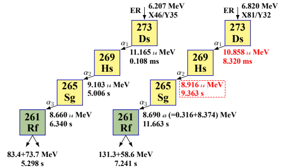
Figure 1: Two complete decay chains assigned to ^{273}\text{Ds} in the ^{238}\text{U}(^{40}\text{Ar}, 5n)^{273}\text{Ds} reaction. For each chain, the energy of the evaporation residue and the corresponding X/Y implantation position are given at the top, followed by the energies of the successive \alpha decays and of the terminal spontaneous-fission event together with the correlation times between adjacent signals. Energies in parentheses indicate summed signals. The numbers written as subscripts after the energies denote the corresponding uncertainties in units of keV. The red entries mark the newly observed branch and the related tentative state assignment discussed in the present work.
