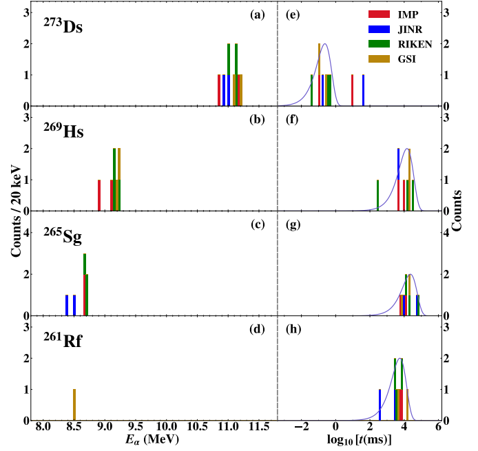
Figure 2: Compilation of the E_\alpha values and decay-time distributions for the decay chains involving ^{273}\text{Ds} , ^{269}\text{Hs} , ^{265}\text{Sg} , and ^{261}\text{Rf} . Panels (a)–(d) show the measured \alpha -particle energies, and panels (e)–(h) show the corresponding distributions of \log_{10}[t(\text{ms})] . The red, blue, green, and yellow histograms represent the data from IMP, JINR [17], RIKEN [15, 16], and GSI [13, 14], respectively. The smooth curves in the decay-time panels are drawn according to Ref. [33].
