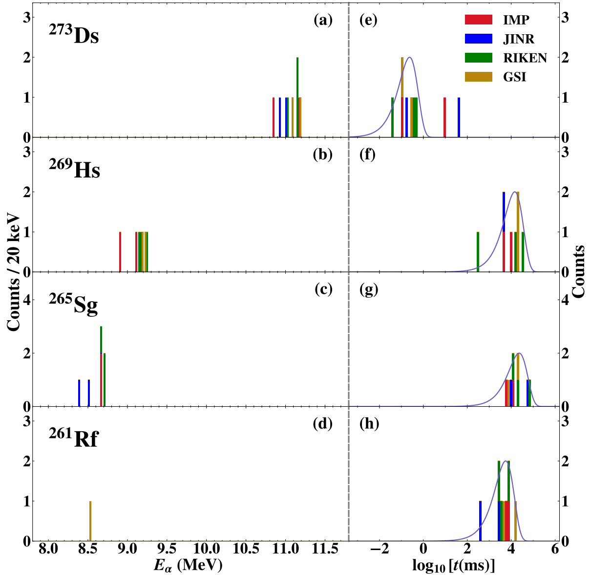
Figure 2: Comparison of the E_\alpha and mean life information for decay chains involving ^{273}\text{Ds} . The red, blue, green, and yellow symbols correspond to the IMP, JINR [2], RIKEN [4, 5], and GSI [3, 6]. The fit curves in the decay-time panels are drawn according to Ref. [7].
