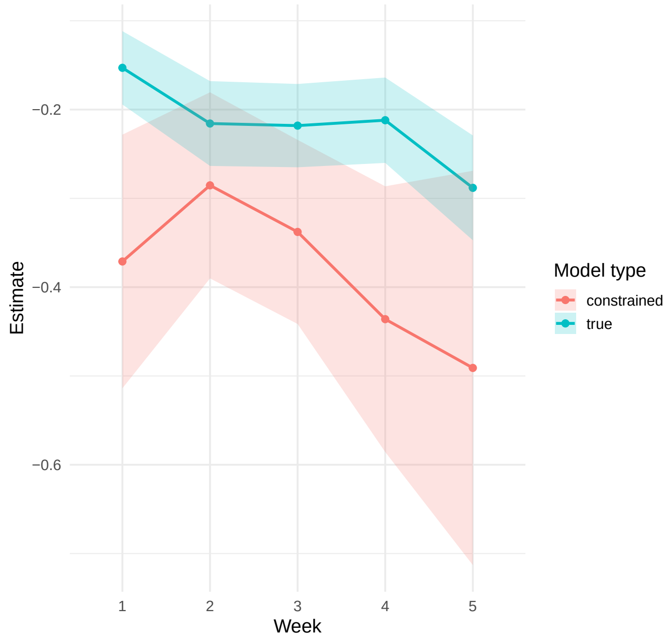
Parameter estimates over time: deference
