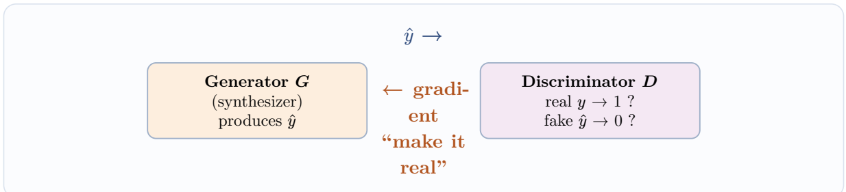
Figure 5: The adversarial game. G wants D to score its output as real; D wants to score real as 1 and fake as 0. They are trained in alternation, each with its own AdamW optimiser.
