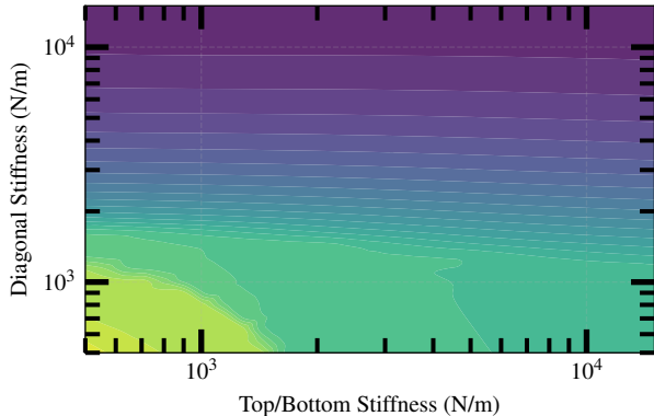
Top/Bottom Stiffness vs Diagonal Stiffness when Left/Right Stiffness = 1000 N/m
