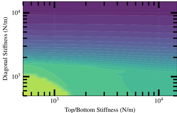
Top/Bottom Stiffness vs Diagonal Stiffness when Left/Right Stiffness = 1500 N/m
