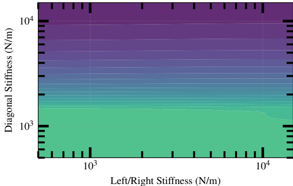
Left/Right Stiffness vs Diagonal Stiffness when Top/Bottom Stiffness = 2000 N/m
