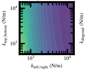
k_{\text{left/right}} VS k_{\text{top/bottom}} when k_{\text{diagonal}} = 1000 \text{ N/m}
