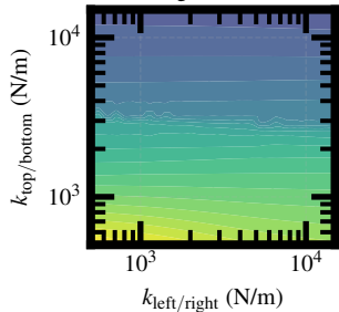
k_{\text{left/right}} VS k_{\text{top/bottom}} when k_{\text{diagonal}} = 500 \text{ N/m}
