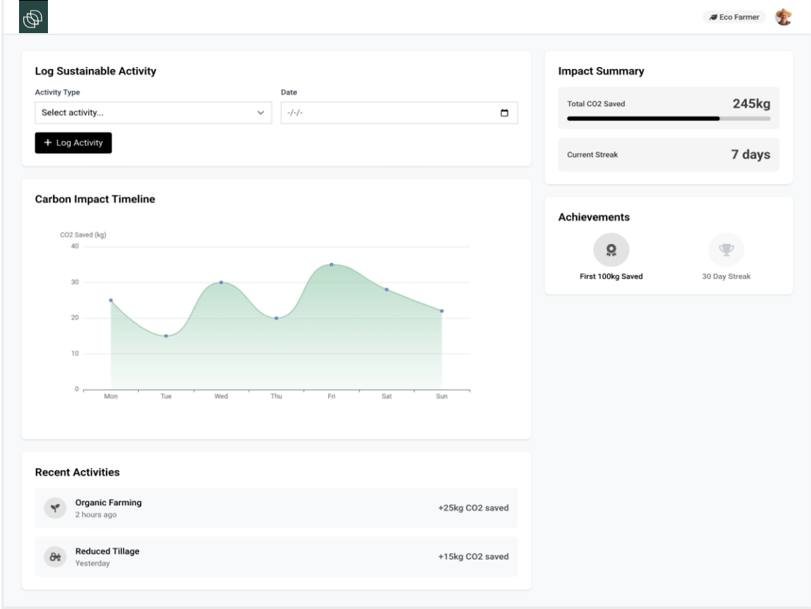
Activity Screen
