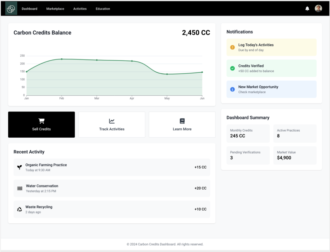
Home Screen
