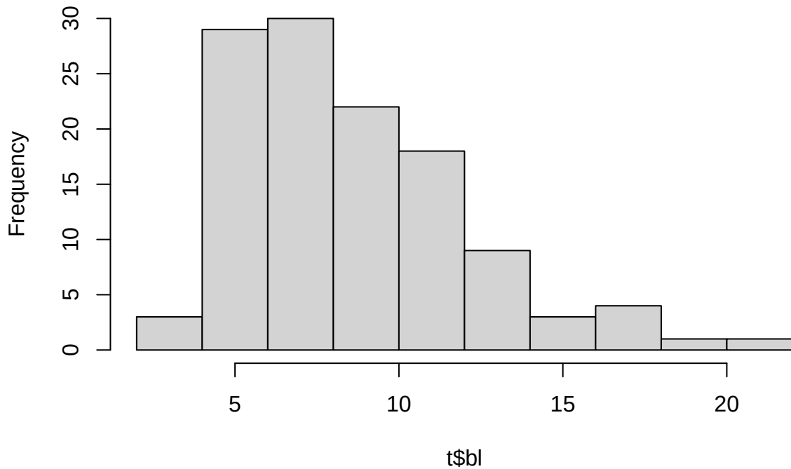
Histogram of t$bl
