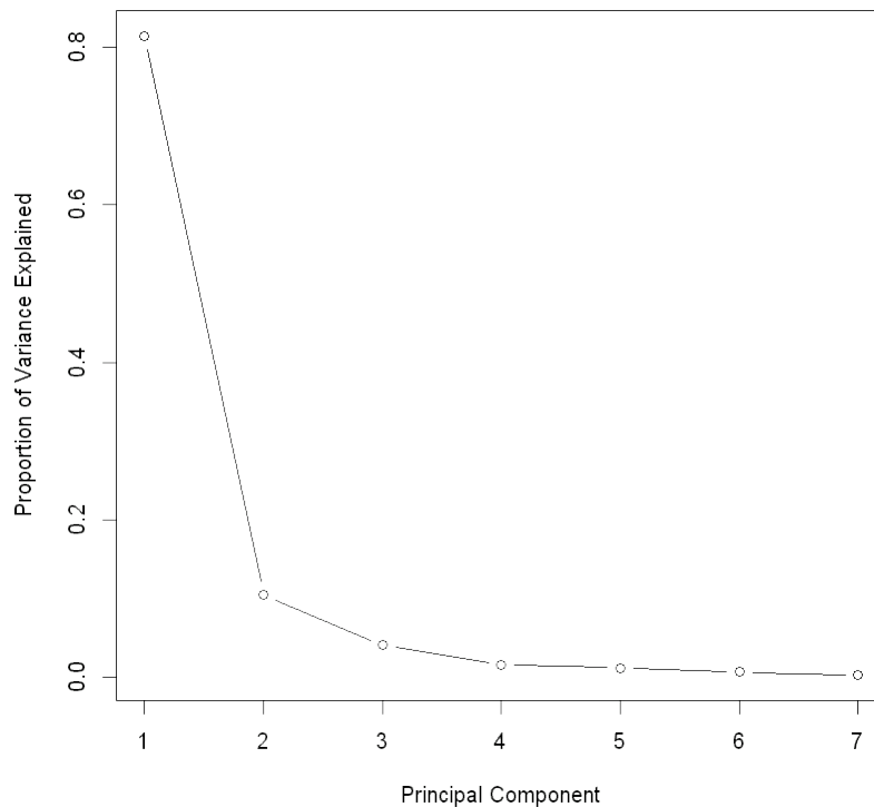
Variance Explained by each PCA component
