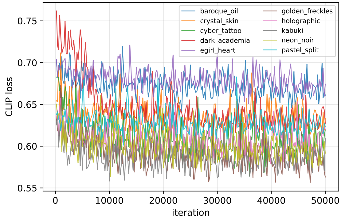
(b) CLIP loss (semantic alignment)
