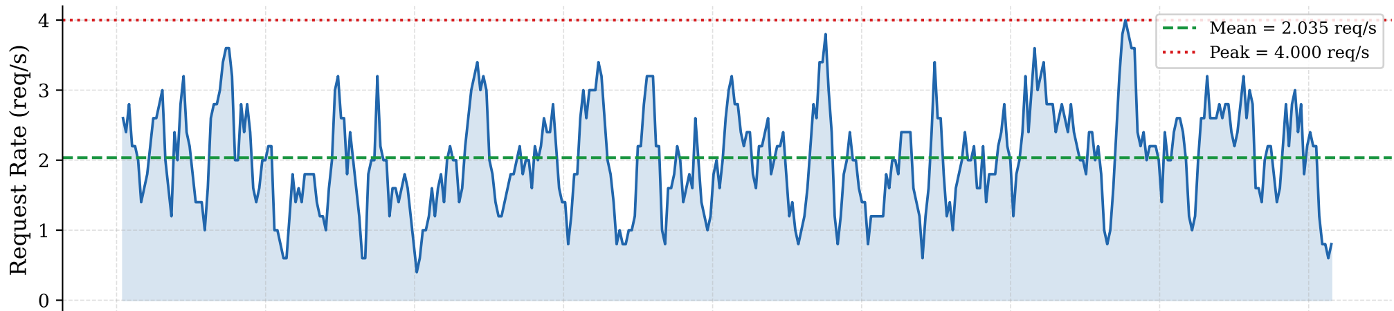
sharegpt_x [rate2.0]: Arrival Rates (window = 5 s)
