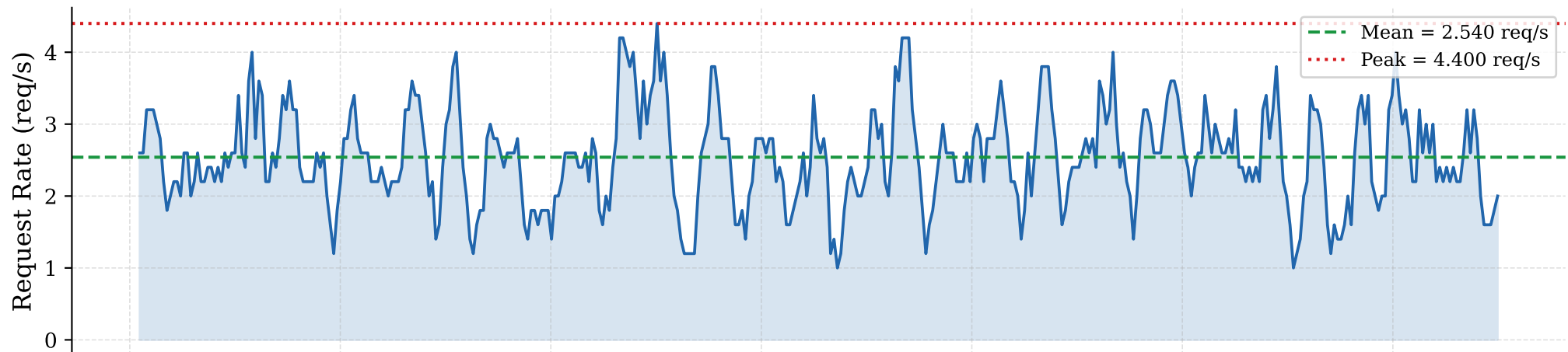
sharegpt_x [rate2.5]: Arrival Rates (window = 5 s)
