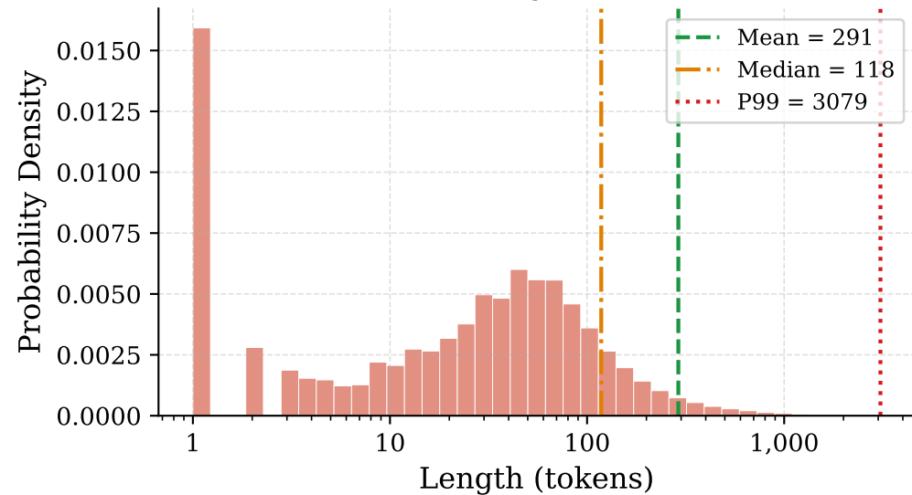
(c) Output Length Distribution
