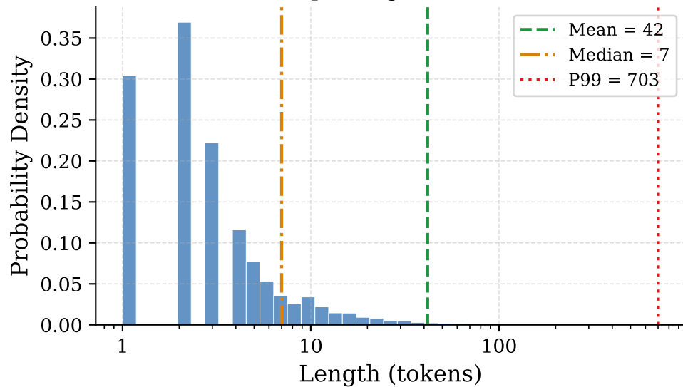
(c) Output Length Distribution
