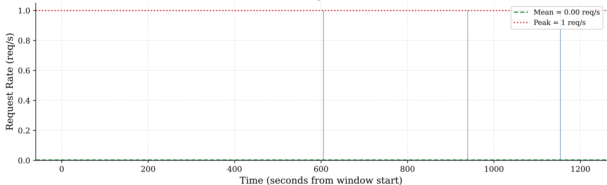
sharegpt_x [low workload]: 1-s Arrival Rate (20-min snapshot) 3 requests
