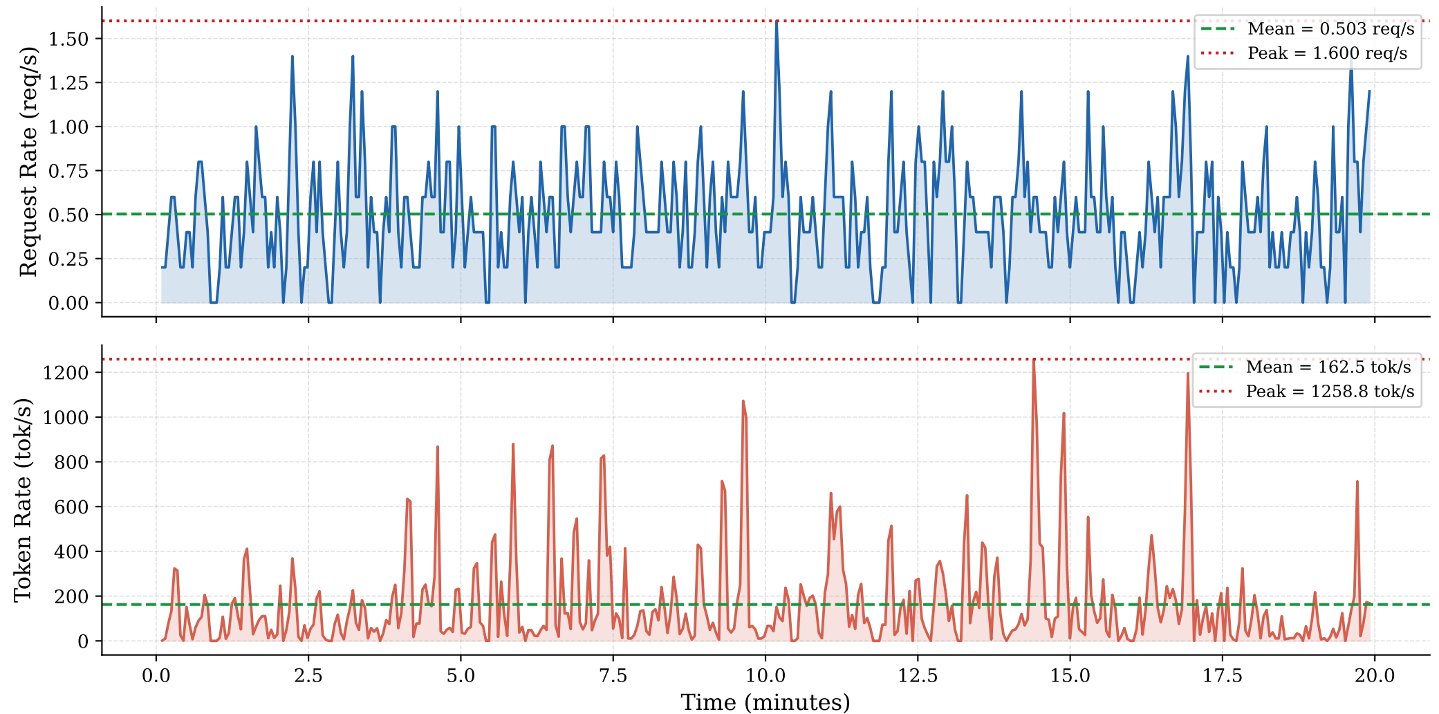
sharegpt_x [rate0.5]: Arrival Rates (window = 5 s, 20-min snapshot)
