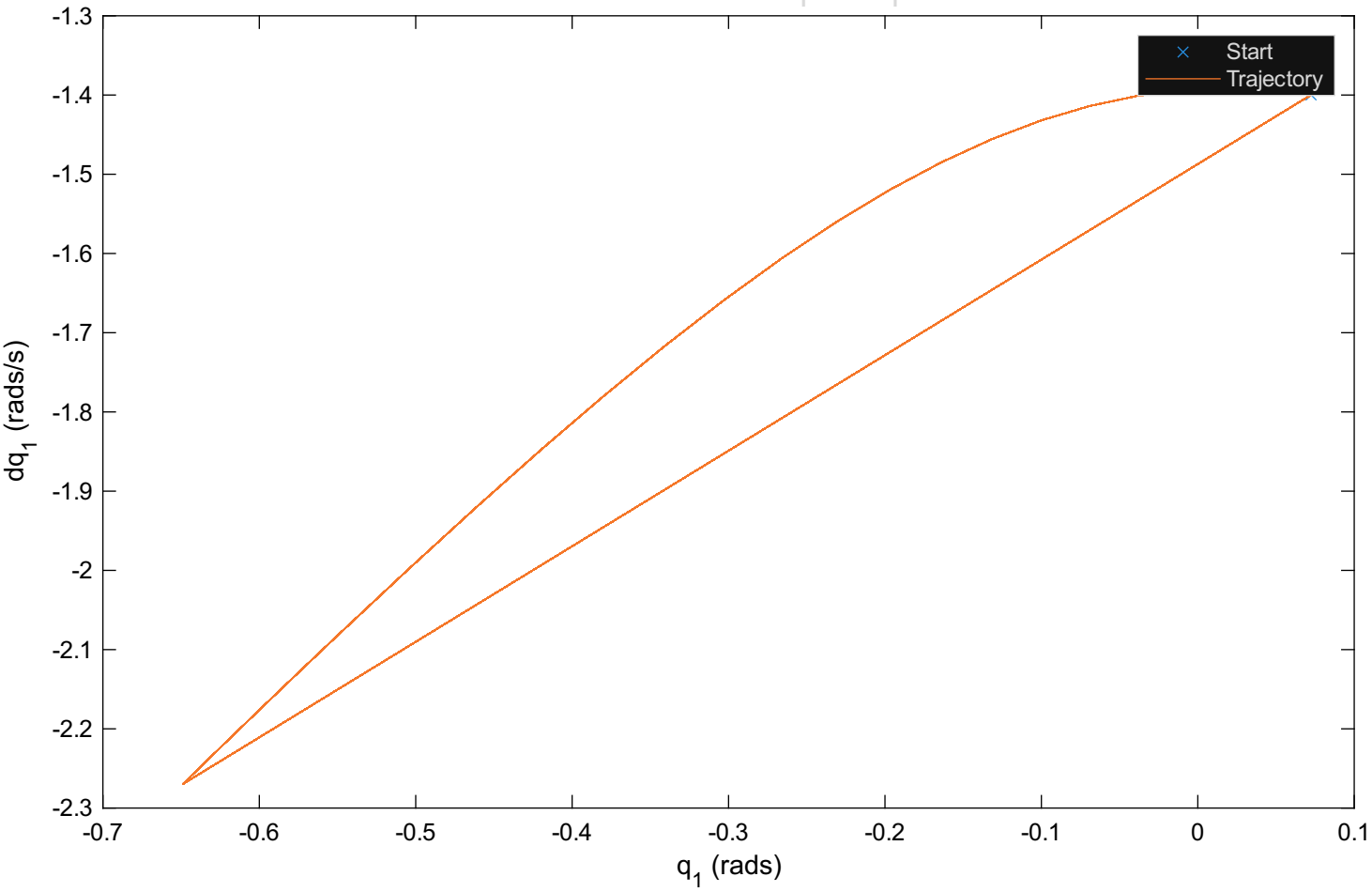
Phase portrait of q_1 vd dq_1
