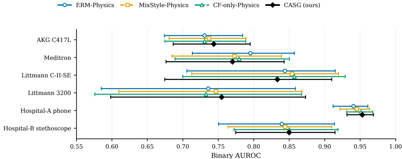
Unseen-device and external-site discrimination (seed ensemble, 95% CI)
