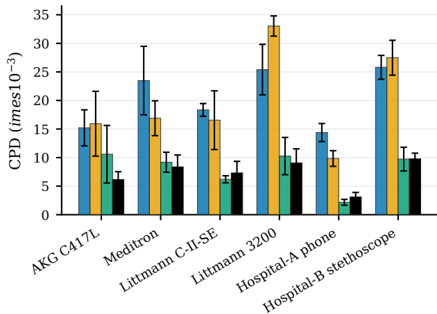
(a) CPD
