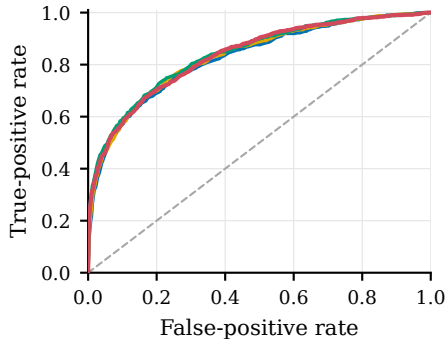
(a) ROC
