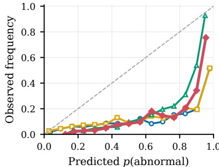
(c) Reliability
