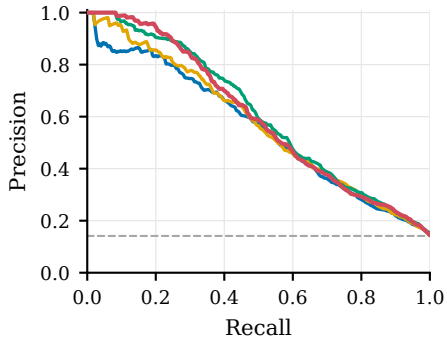
(b) Precision-recall
