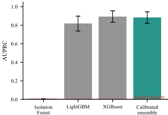
Base models vs ensemble (mean \pm std)
