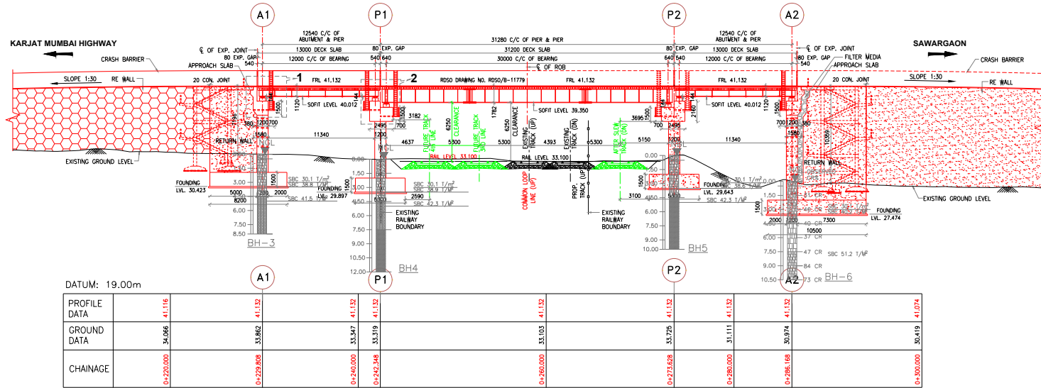
HALF ELEVATION & HALF SECTIONAL A-A (Along C/L of Proposed Alignment)
