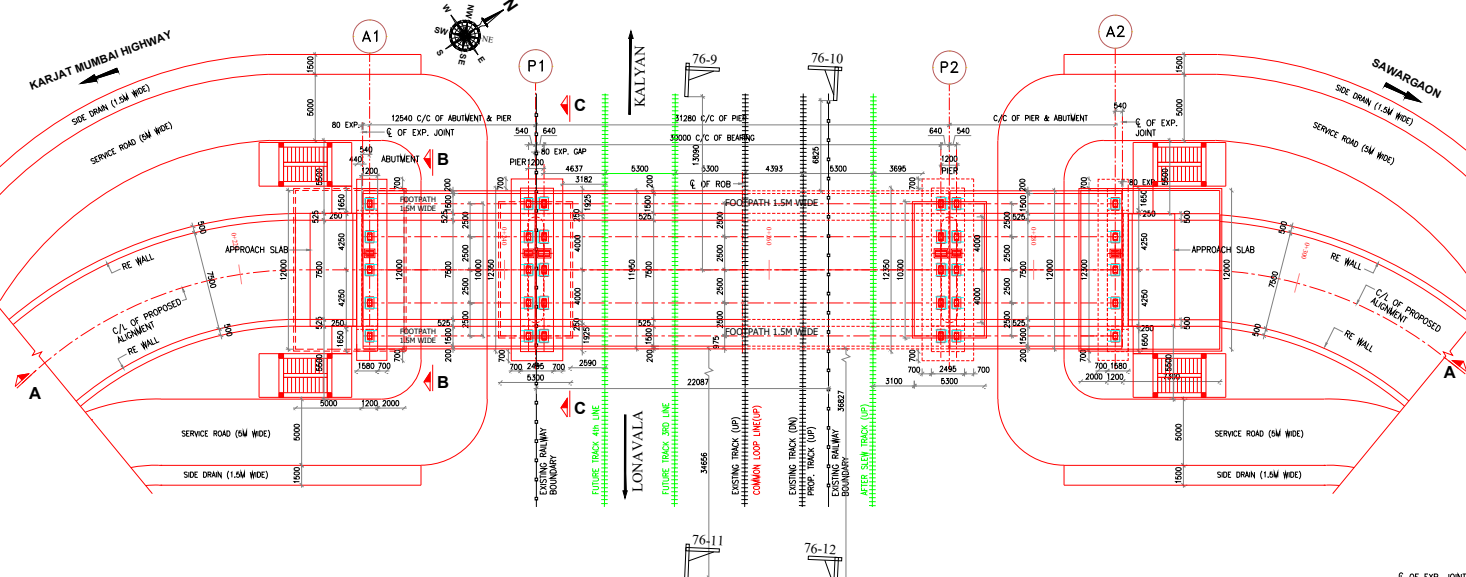
HALF TOP & HALF BOTTOM PLAN
