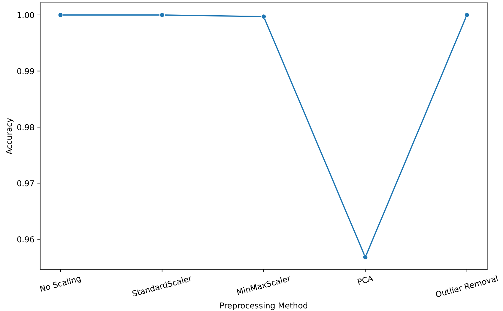
Effect of Preprocessing on Model Accuracy
