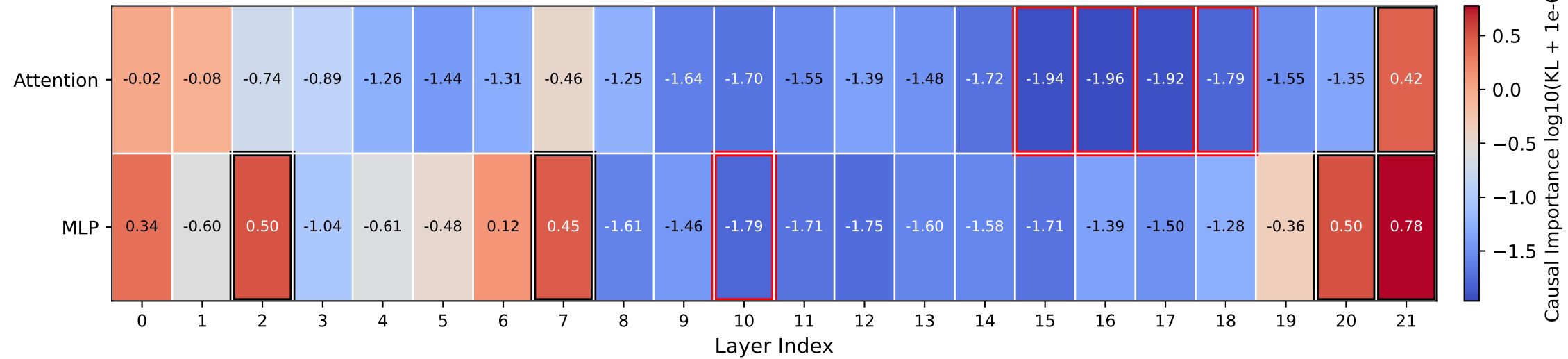
Module-Level Causal Importance in TinyLlama-1.1B (Log Scale)
