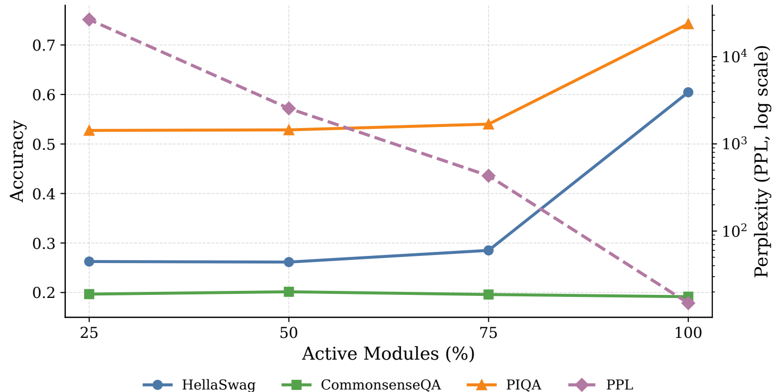
Effect of Active Module Ratio on Model Performance
