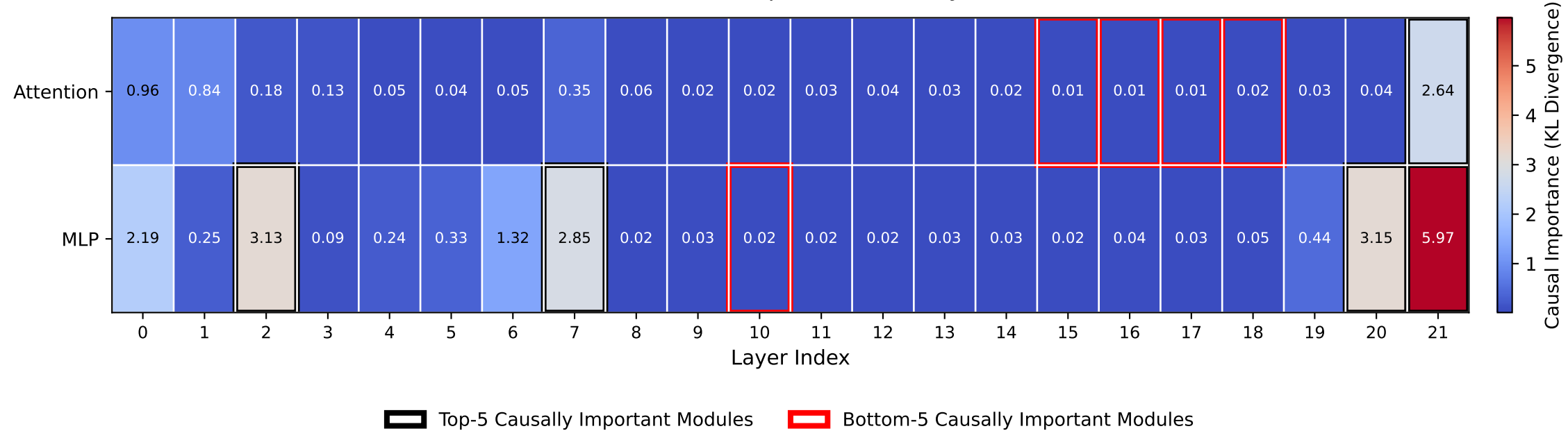
Module-Level Causal Importance in TinyLlama-1.1B
