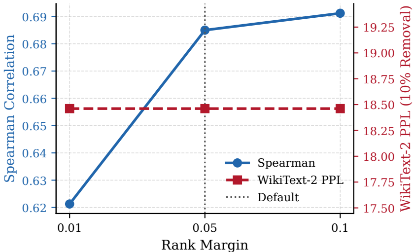
Sensitivity to Rank Margin
