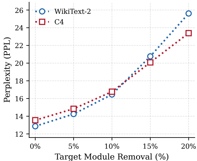
(a) Qwen2.5-3B-Instruct
