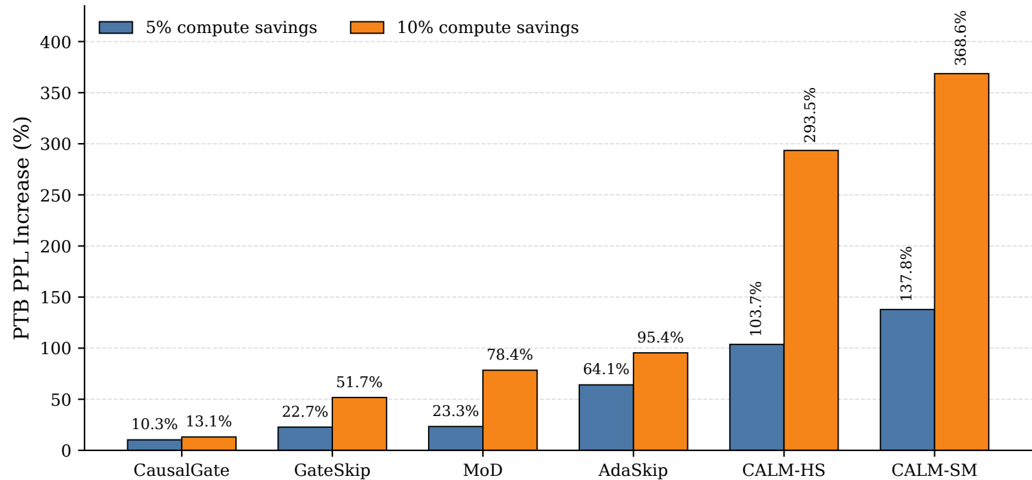
Relative PTB Perplexity Degradation
