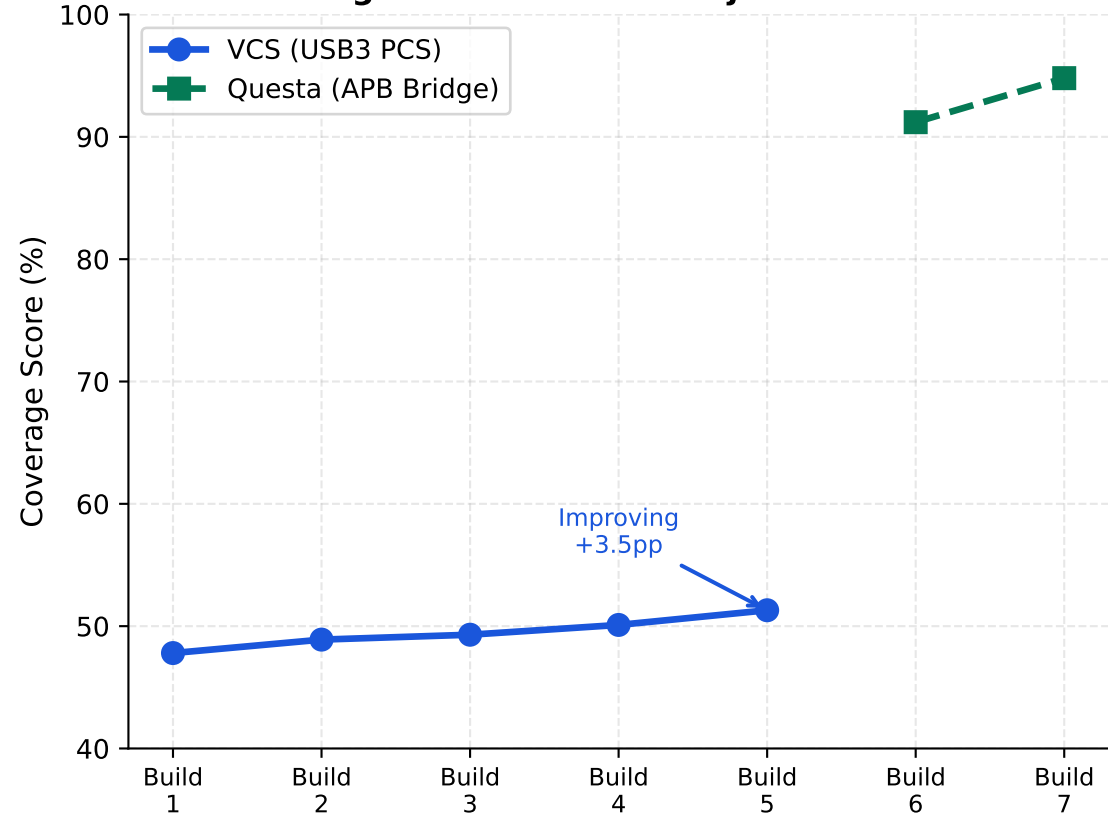
coverage.trend — Multi-Project CI Timeline
