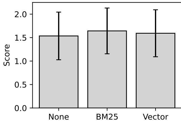
Security Specificity
