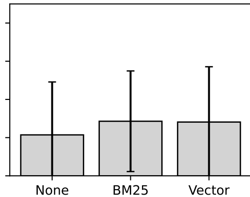
Hallucination (inv.)
