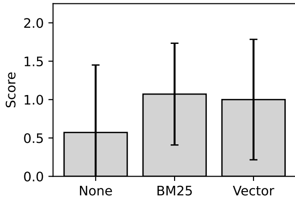
Security Specificity
