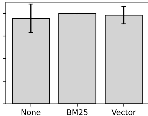
Hallucination (inv.)
