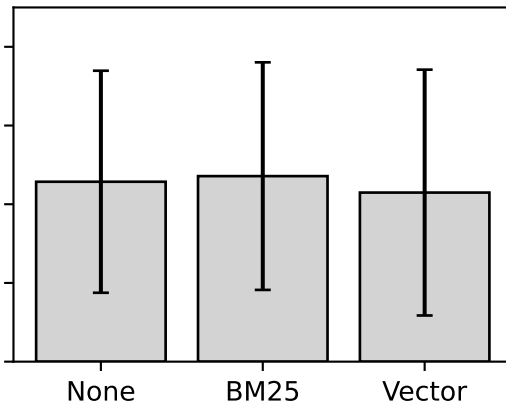
Context Utilization
