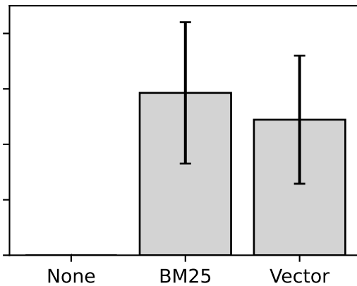
Context Utilization
