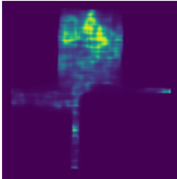
Generated Label
