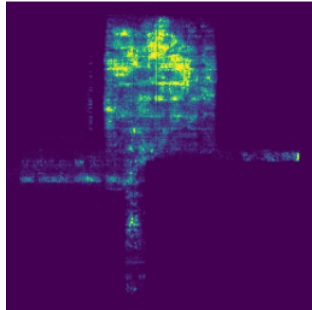
Ground Truth
