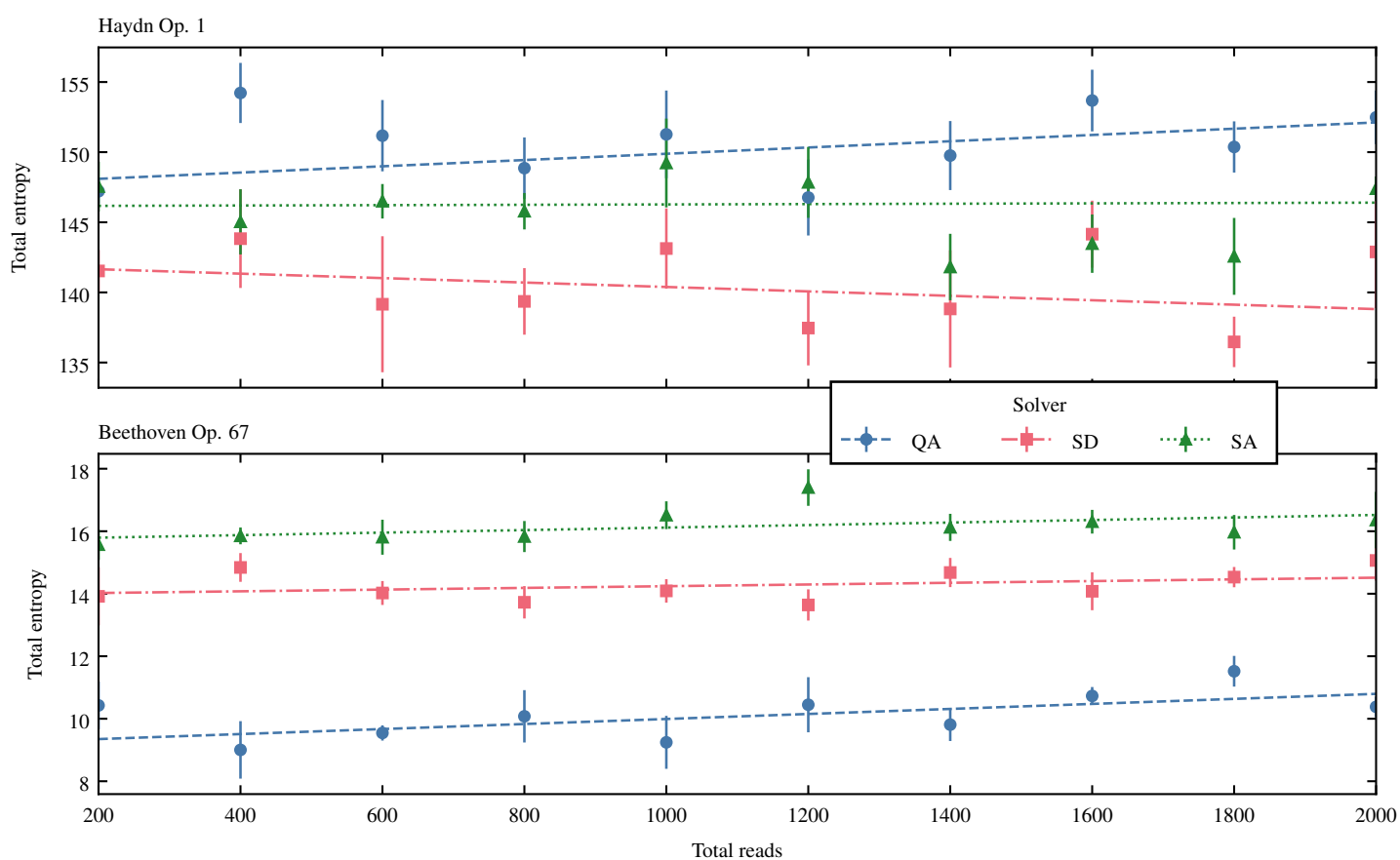
Figure 9: Comparison between quantum annealing (QA), steepest descent (SD), and simulated annealing (SA) entropies of the same lowest-energy samples as Fig. 8. Best-fit lines found via a least-squares regression.
