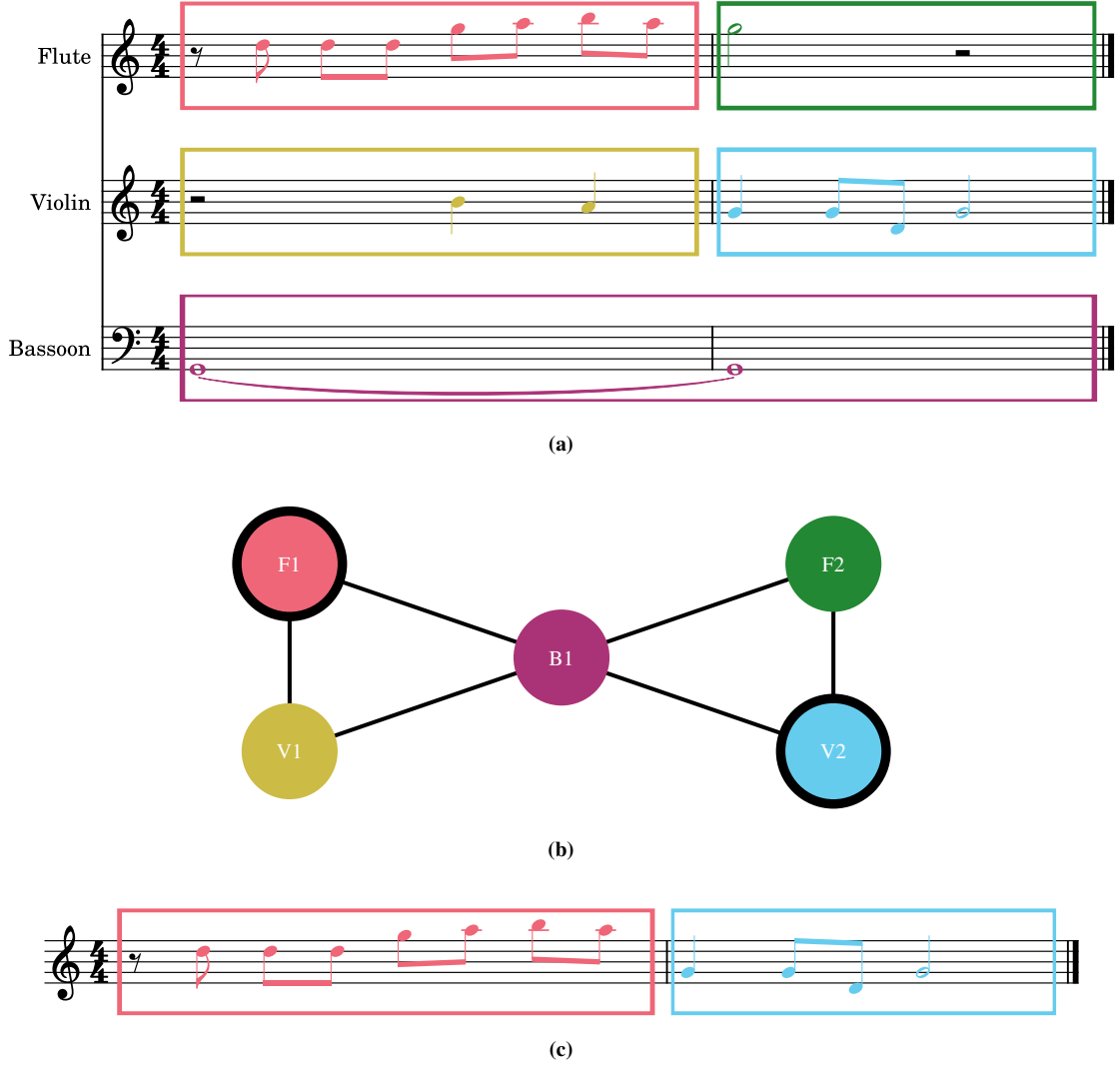
Figure 2: Toy example demonstrating a simplified version of the proposed framework. (a) Example score of three parts. Phrases identified by the LBDM have been coloured and outlined. (b) Graph of the score, with the colour and label of each vertex corresponding to its phrase, and edges connecting overlapping phrases. One possible solution of proper vertex colouring, with n = 1 , is shown by the outlined vertices. (c) Score representation of the final arrangement.
