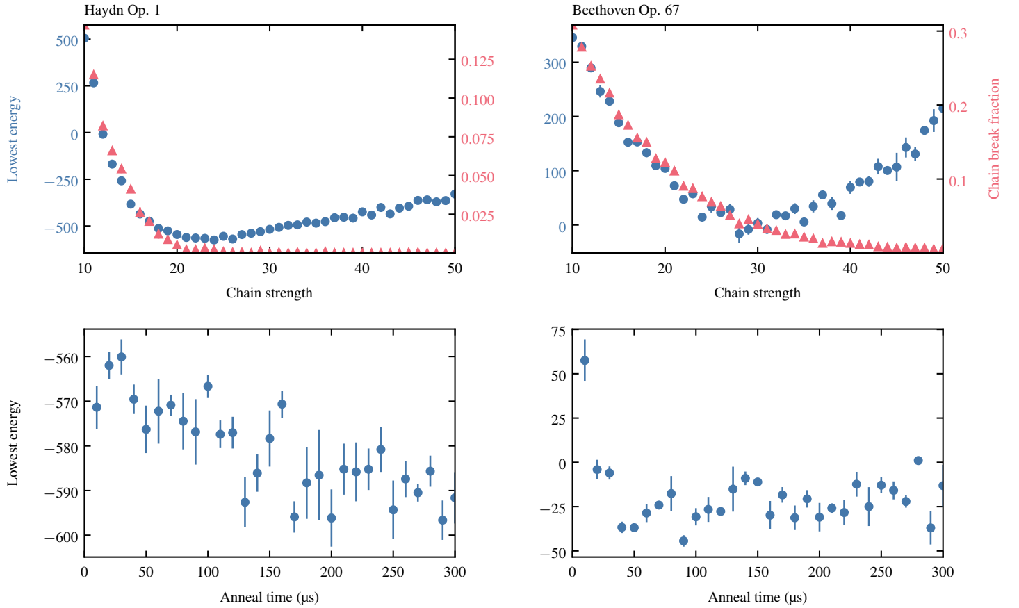
Figure 7: Optimisation of the solver configuration. Each data point sampled three times at 1000 reads, with the mean and standard error calculated. Same n as Fig. 6. (Top) Variation of the fraction of chains broken (red triangles) and energy (blue circles) of the lowest-energy samples with chain strength, using the default anneal time (20 \mu s). (Bottom) Variation of lowest energy with anneal time per sample, using the updated chain strength.
