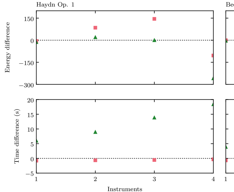
Figure 10: Comparing solutions returned by steepest descent (red squares) and simulated annealing (green triangles) against quantum annealing. Each data point sampled five times at 2000 reads, with the mean and standard error calculated. Difference from quantum annealing shown, with a positive difference signifying an advantage towards quantum annealing. (Top) Lowest-energy samples of the returned sample set. (Bottom) Time to solution, in seconds.
