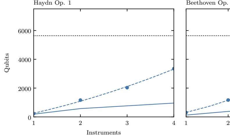
Figure 4: Number of qubits required for problems of different instruments, with the dotted line marking the maximum number of accessible qubits in a D-Wave QPU (5640). Logical qubits (equivalent to the number of variables) shown as solid lines, physical qubits required to embed the problem shown as points with a dashed line quadratic fit. Shaded region represents a theoretical extrapolation to arrangement for a higher number of instruments.
