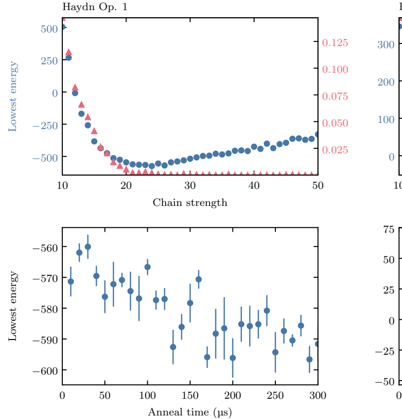
Figure 7: Optimisation of the solver configuration. Each data point sampled three times at 1000 reads, with the mean and standard error calculated. Same n as Fig. 6. (Top) Variation of the fraction of chains broken (red triangles) and energy (blue circles) of the lowest-energy samples with chain strength, using the default anneal time (20 \mu s). (Bottom) Variation of lowest energy with anneal time per sample, using the updated chain strength.
