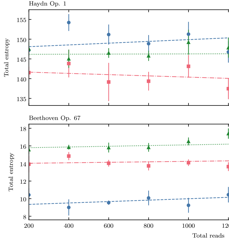
Figure 9: Comparison between quantum annealing (QA), steepest descent (SD), and simulated annealing (SA) entropies of the same lowest-energy samples as Fig. 8. Best-fit lines found via a least-squares regression.
