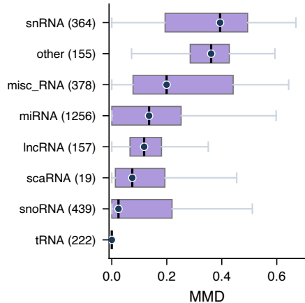
MMD by biotype
