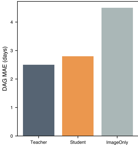
A. Distillation Performance
