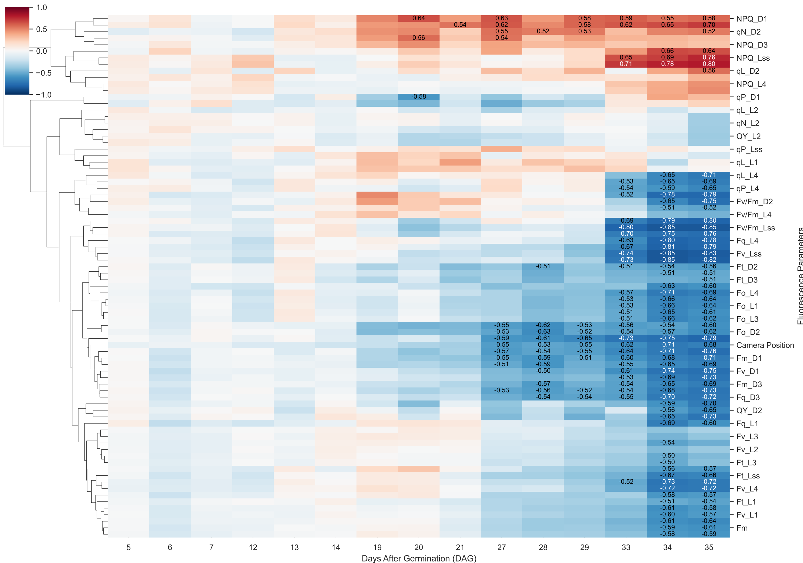
Spearman Correlation Between Fluorescence Parameters and Drought Treatment
