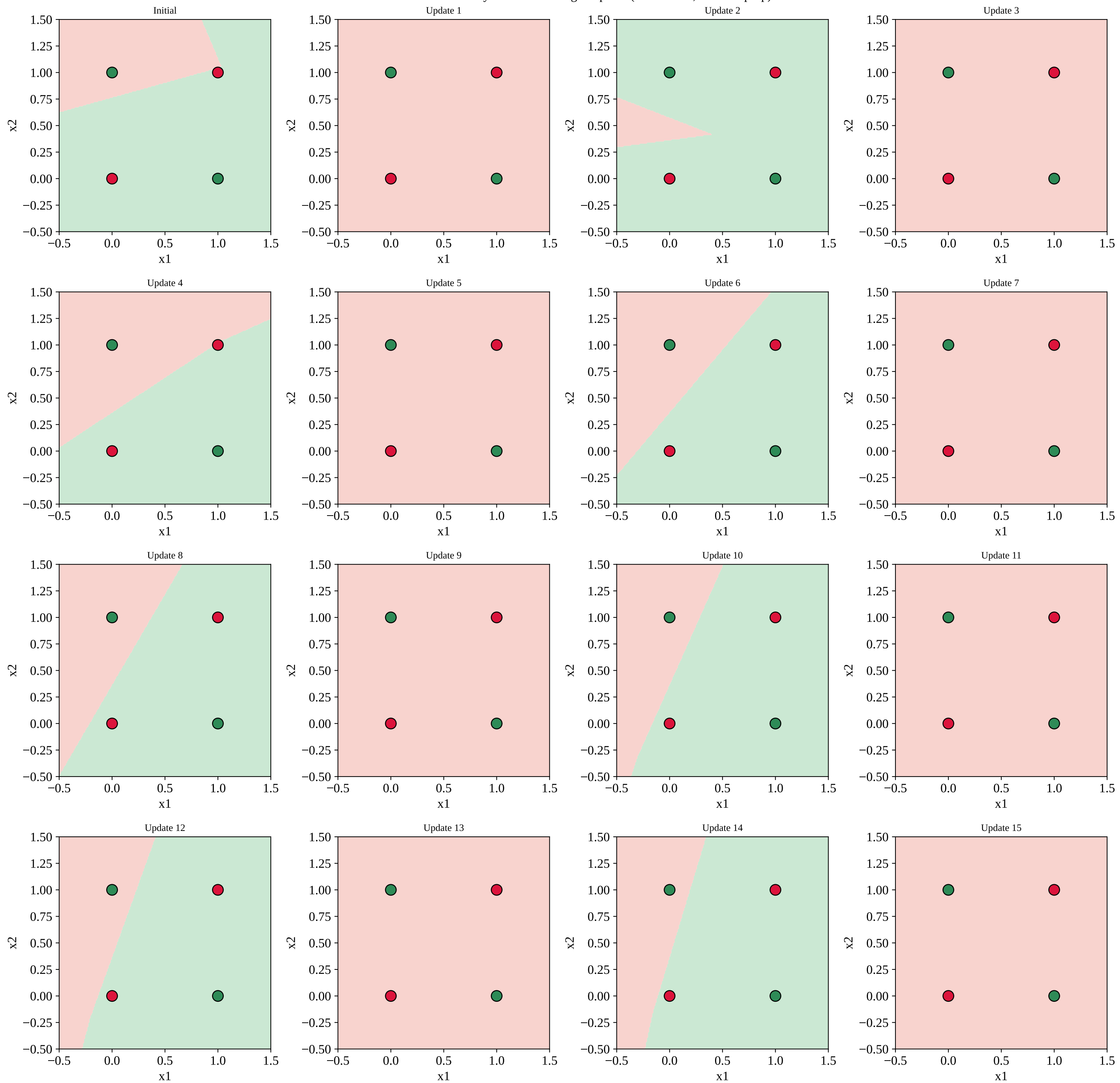
XOR: Decision Boundary After Each Weight Update (Naive MLP, No Backprop)
