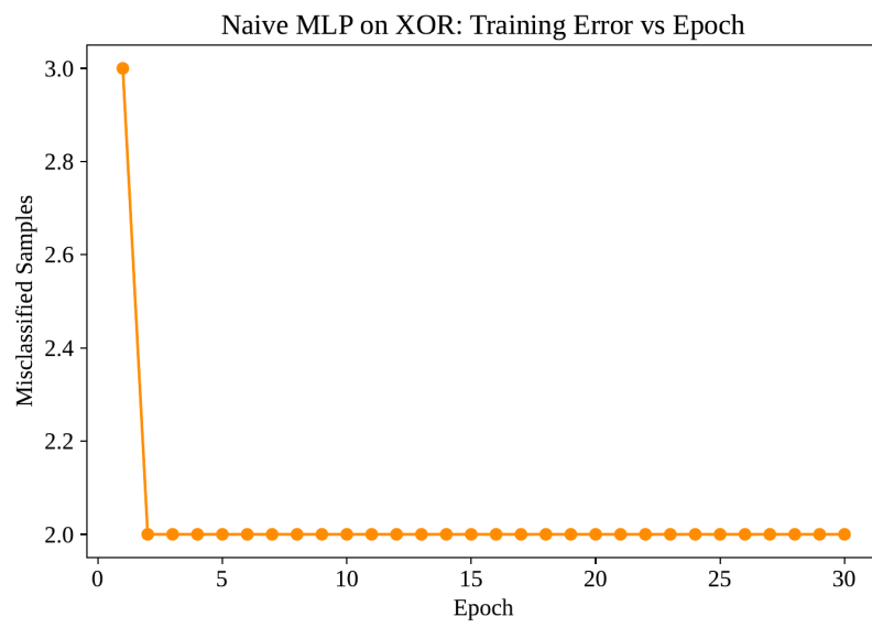
Figure 2: Naive MLP - training error stuck at 2/4.
