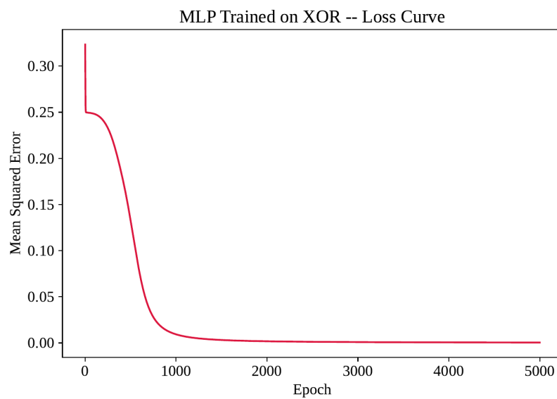
Figure 5: Loss curve - MSE decays smoothly to ~0.
