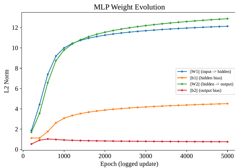
Figure 6: Weight L2 norms settle into a stable set.
