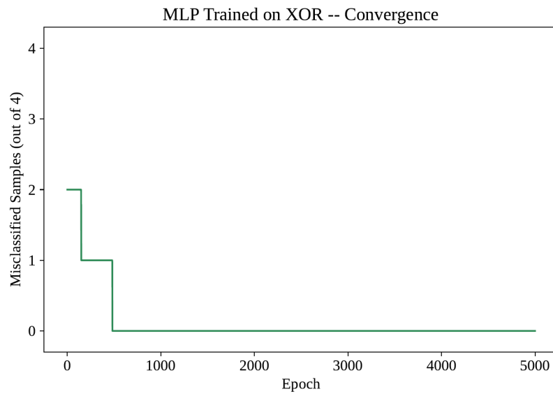
Figure 4: Convergence - misclassified drops to 0/4 and stays.
