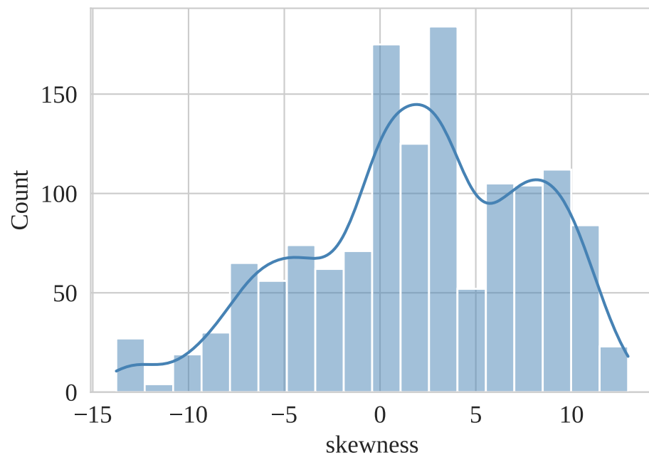
Distribution of skewness
