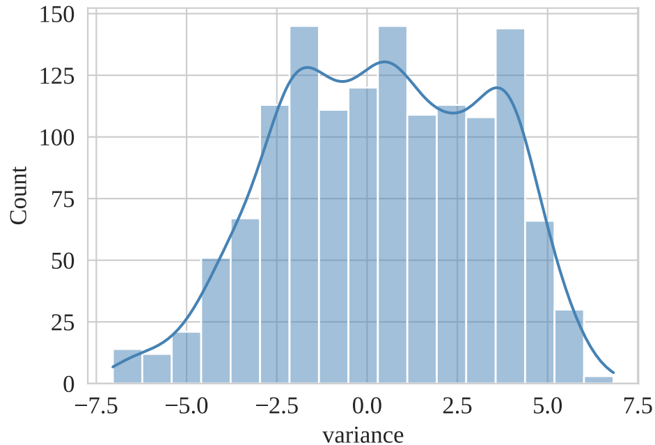
Distribution of variance
