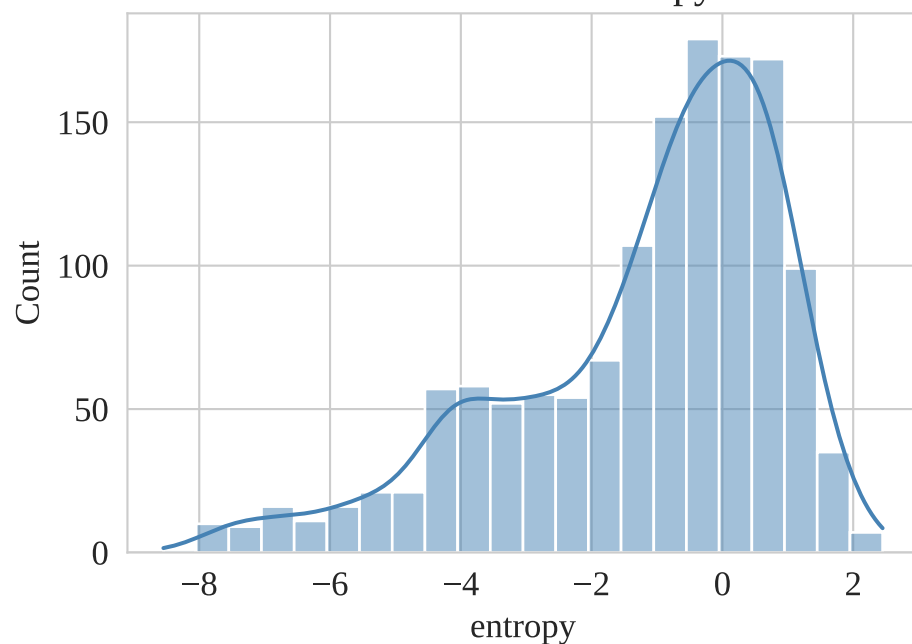
Distribution of entropy
