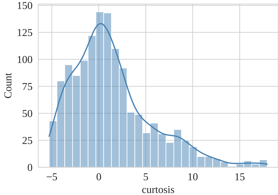
Distribution of kurtosis
