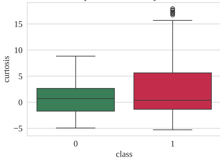
Boxplot of kurtosis by class
