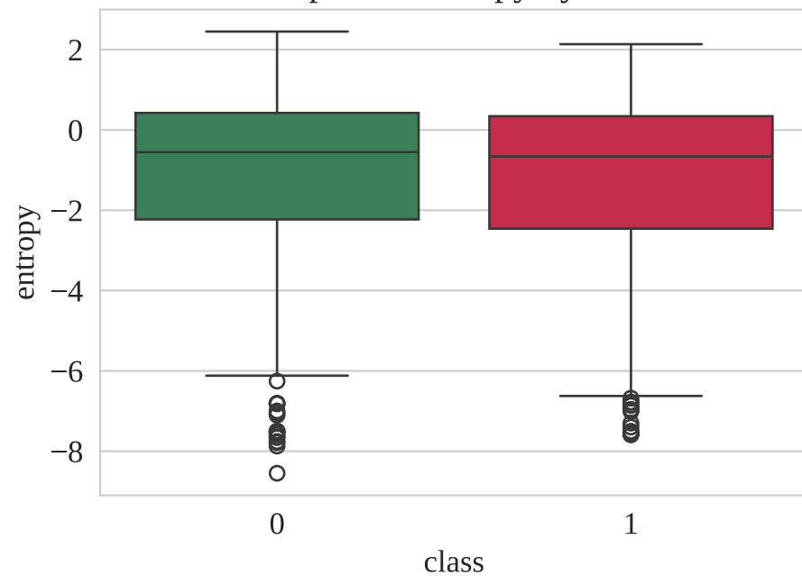
Boxplot of entropy by class
