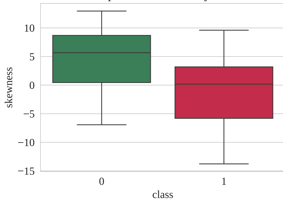
Boxplot of skewness by class
