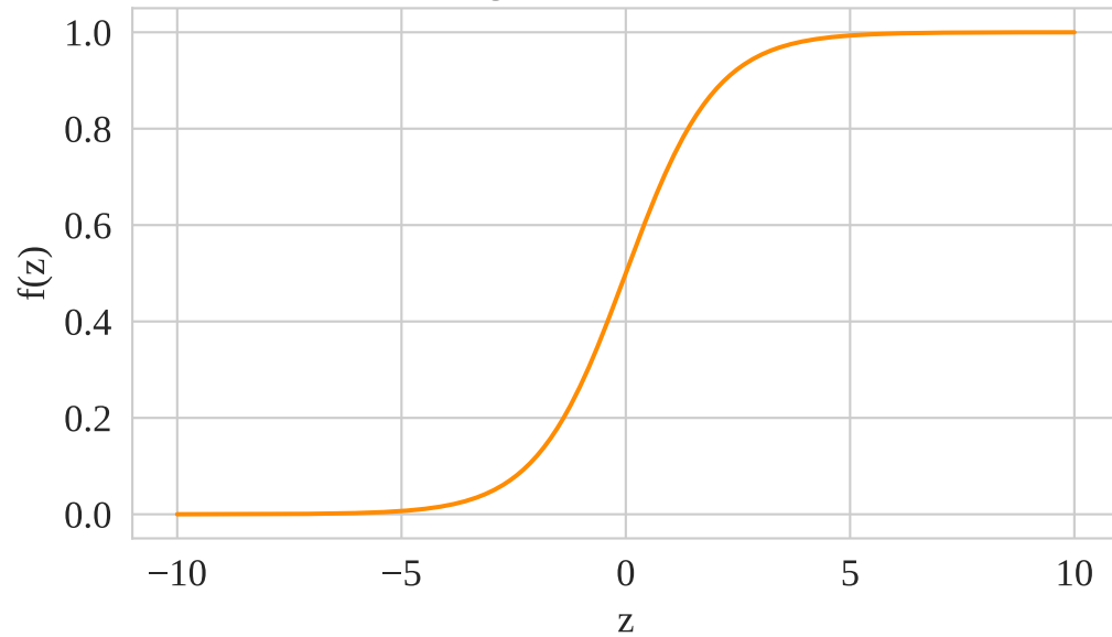
Sigmoid Activation
