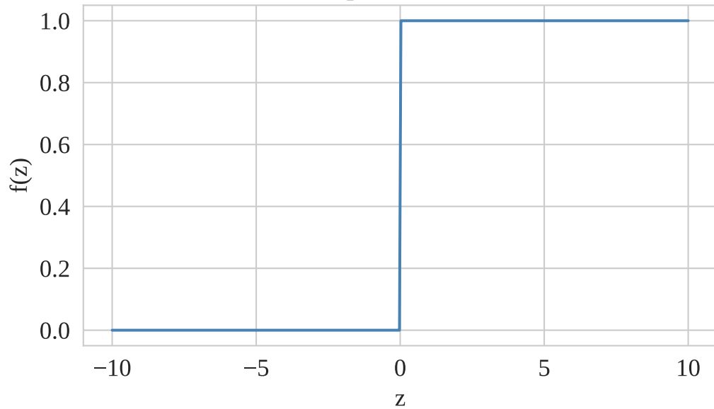
Step Activation
